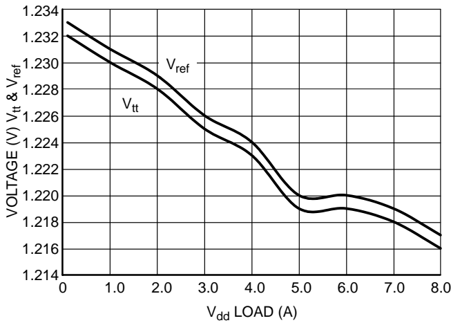
Figure 6. V tt and V ref vs. V dd Load
